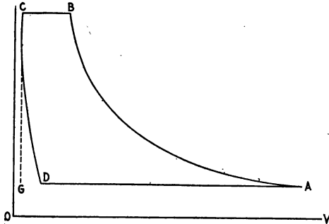
FIG. 43.—Ideal card for piston compressor.
